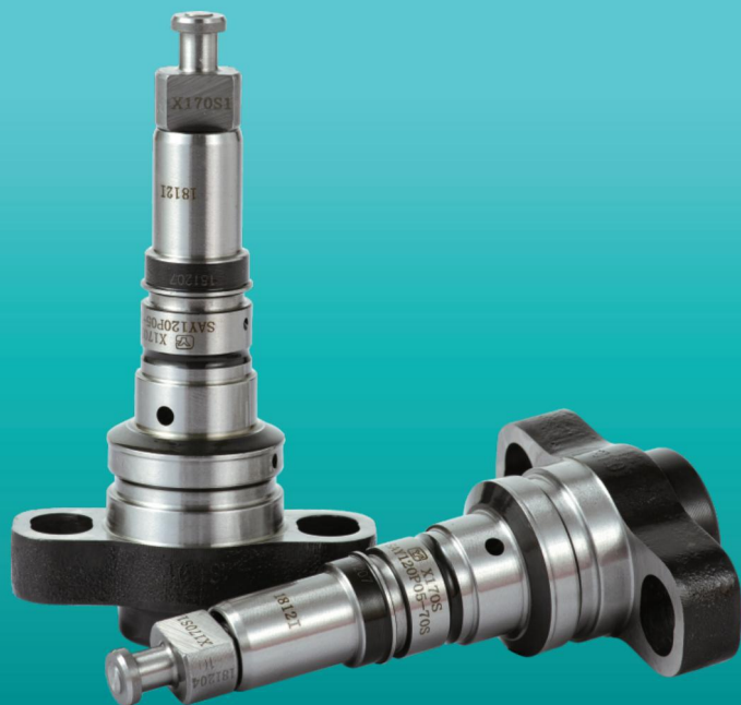
P型泵柱塞副 P type pump barrel&plunge
